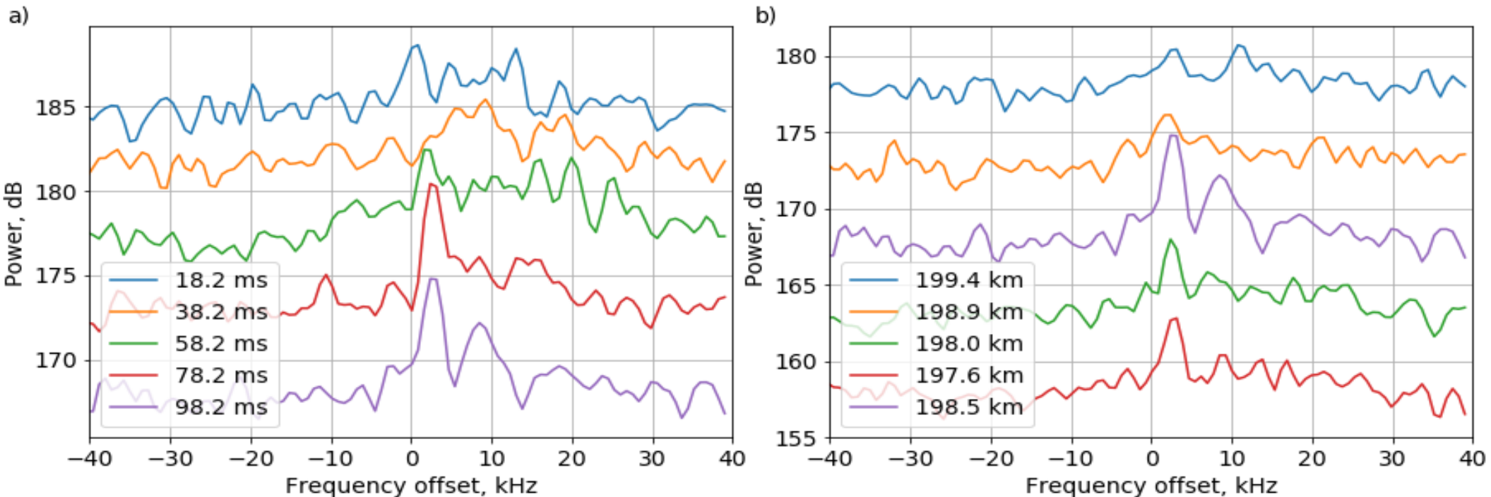
Figure 3. The dynamics of the downshifted plasma line spectra at the stage of Langmuir turbulence development for different pumping times with a step of 20 ms at a fixed height h = 198.5 km (panel a)) and the altitude distribution with a step of 450 m of spectral intensity towards the end of the PW pulse t = 98.2 ms (panel b)). Averaging over 50–55 PW pulses was carried out. An additional shift of each of the spectra by 5 dB was used. 11/08/2018, 15:51:30–16:11:30 LT.
