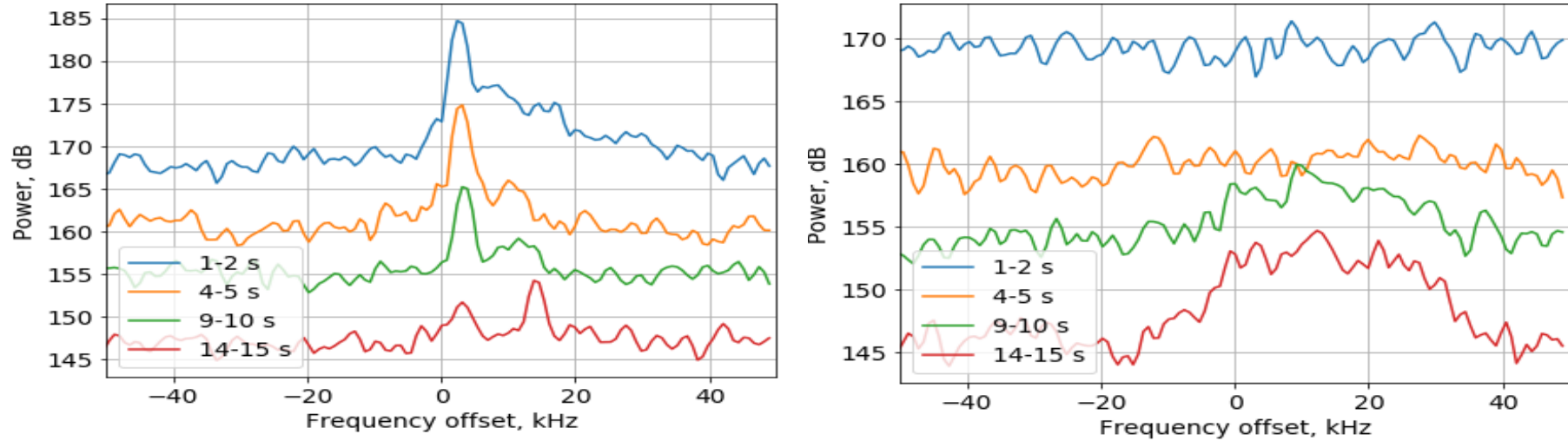
Figure 4. The dynamics of the development of the downshifted plasma line spectra during prolonged quasi-continuous heating for different exposure times (time shift \sim 5 s) at two fixed heights h_1 = 214 km (panel a)) and h_2 = 210.8 km (panel b)). Averaging over 50–55 PW pulses was performed out. An additional shift of each spectra by 5 dB was used. 11/08/2018, 17:46:00–17:46:15 LT.
