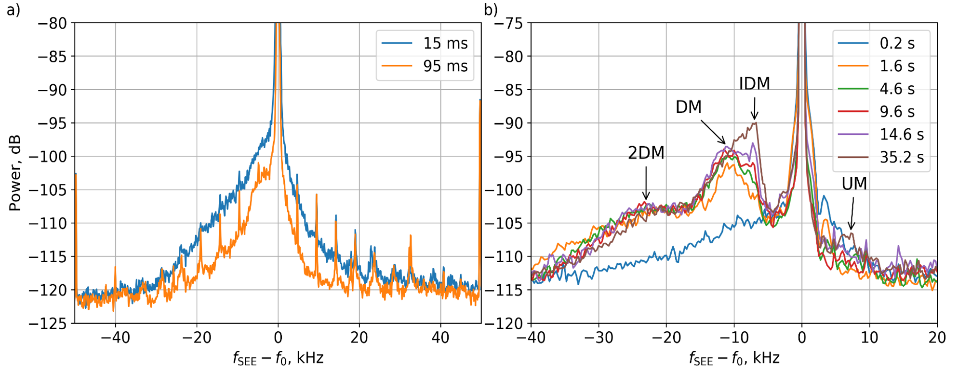
Figure 5. The panel (a): the narrow band ponderomotive narrow continuum SEE feature for the 15 th and 95 th ms of pumping, 55 pulses are averaged, the frequency resolution is 100 Hz. The panel (b): the SEE spectra dynamics for a quasi-continuous radiation mode, the frequency resolution of 250 Hz. The data of 11/08/2018.
