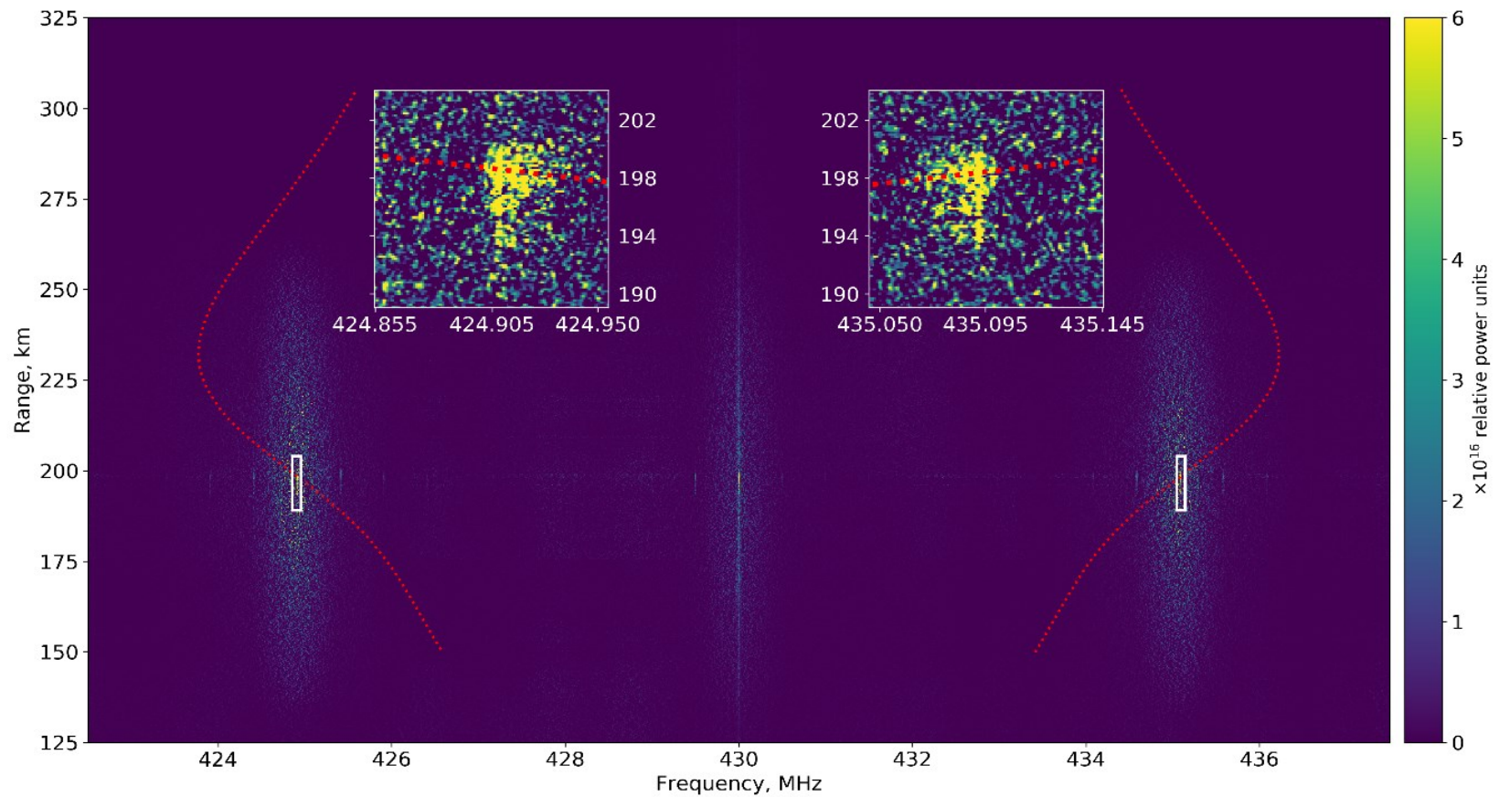
Figure 2. Electron density profile and spectrogram of artificial ion and plasma lines (downshifted plasma line on the left, upshifted plasma line on the right for 98.2 ms of pumping). Separate (zoomed) panels show the region of generation of the plasma line with a high frequency-altitude resolution. 11/08/2018, 15:51:00–16:11:30 LT
