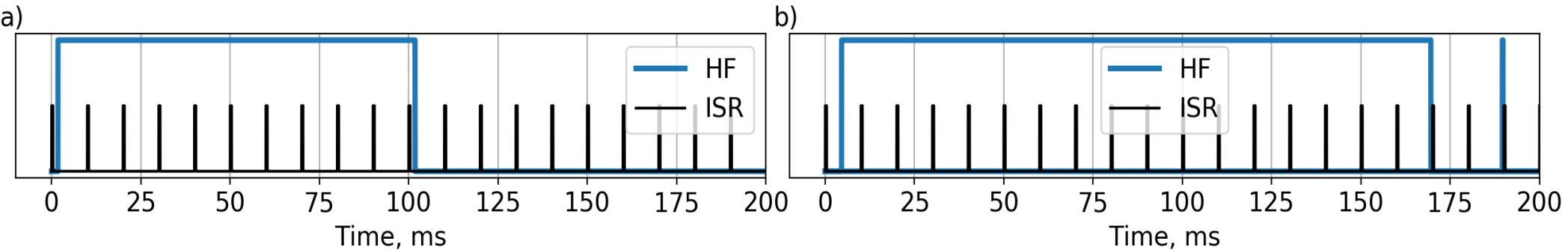
Figure 1. The example of the radiation modes of the heating facility and incoherent scattering radar used in the experiment.
