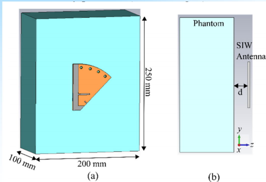
Designed antenna with the single layer body phantom: a) 3D view; b) side view.
